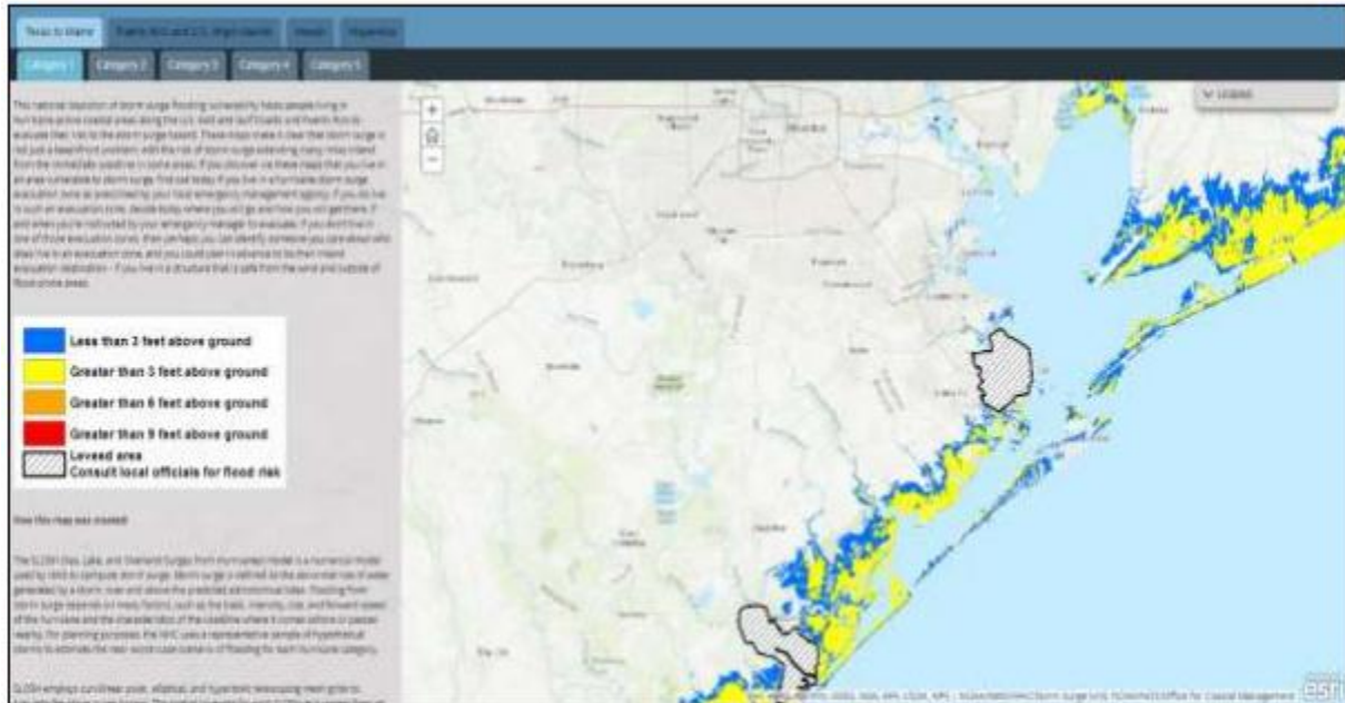
Picture 2 Storm Surge Category 1 Hurricane
