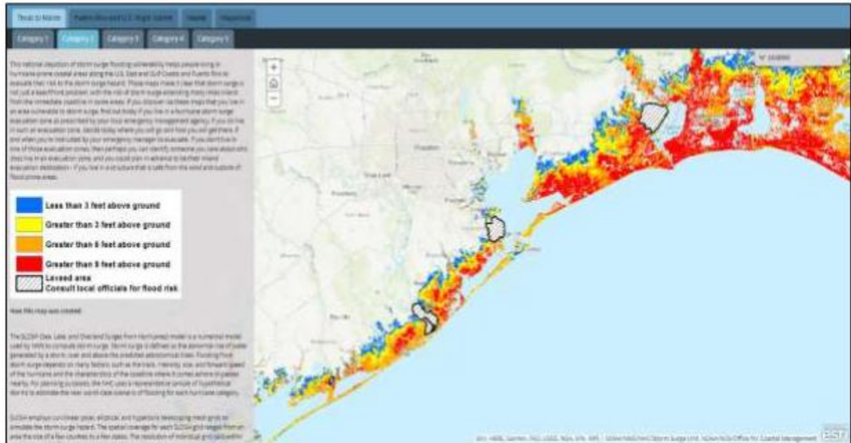
Picture 3 Storm Surge Category 2 Hurricane
