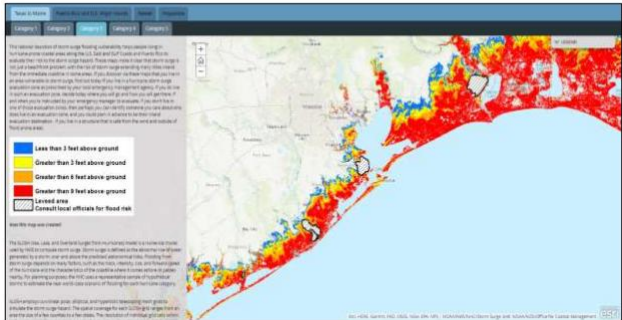
Picture 4 Storm Surge Category 3 Hurricane
