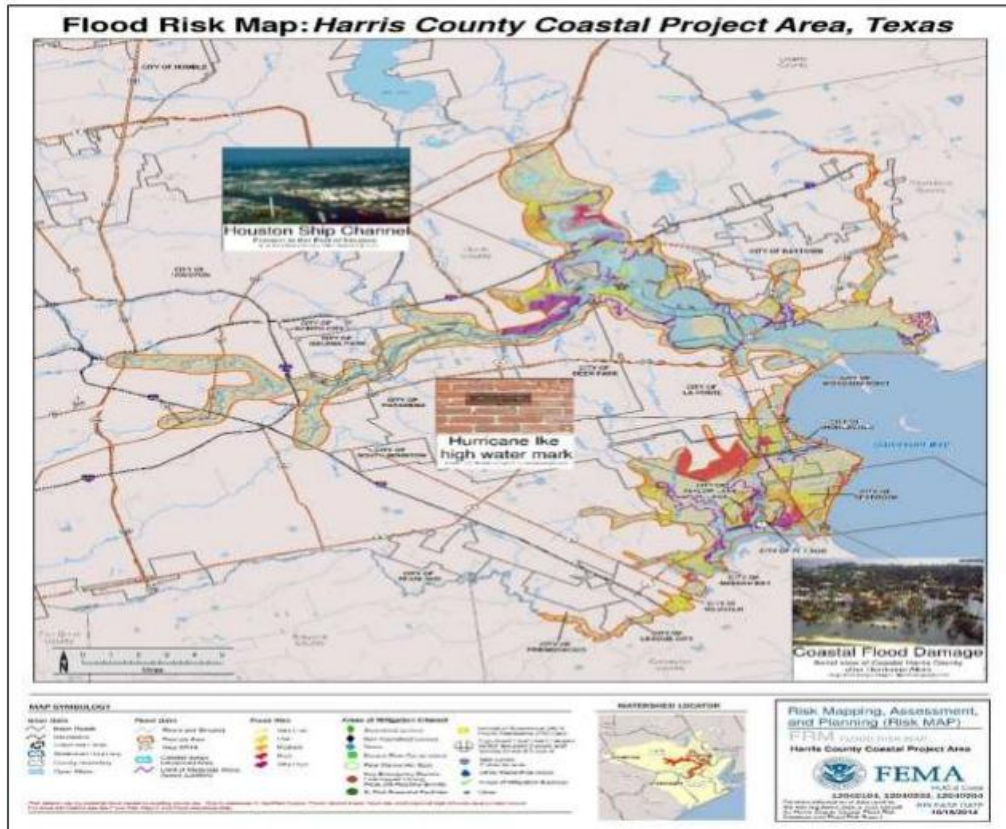
Picture 7 Flood Information Map
