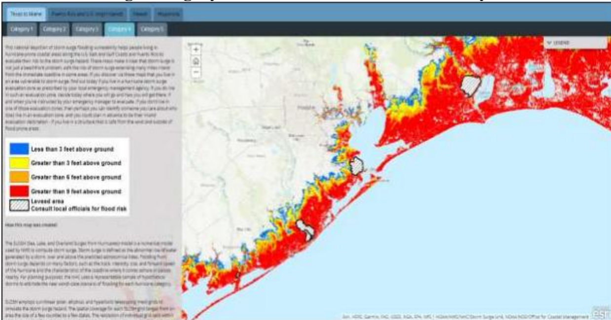
Picture 5 Storm Surge Category 4 Hurricane
