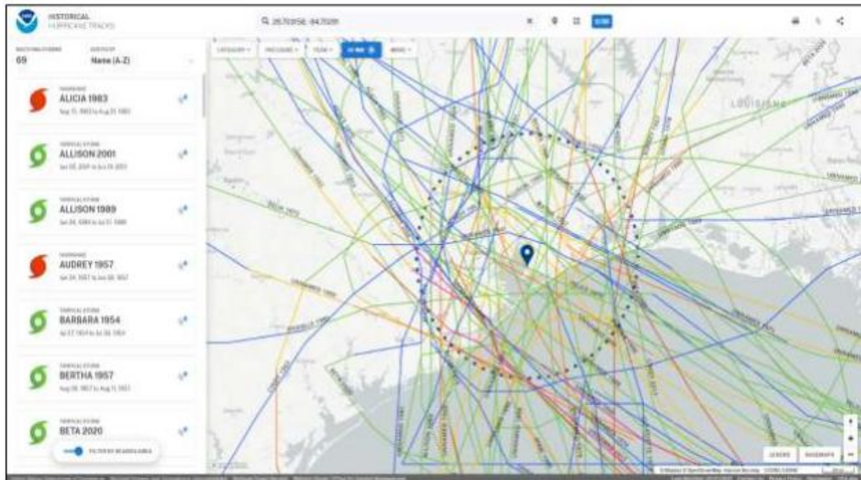
Picture 1 Historical Hurricane Landfall Data
